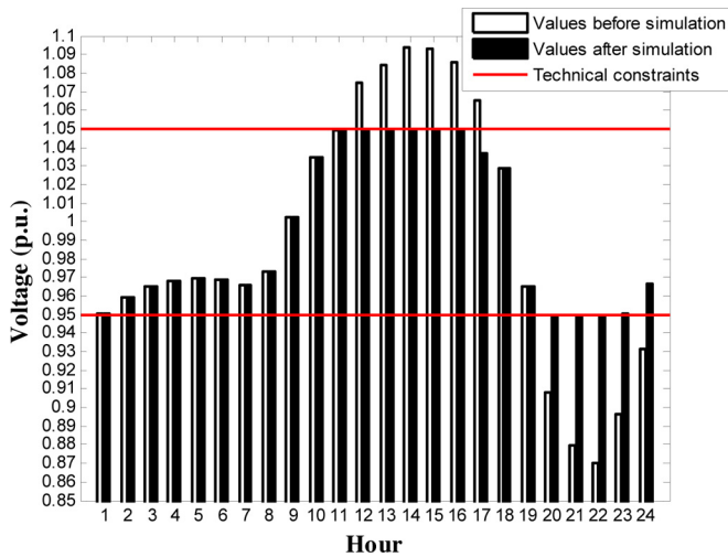
Fig. 6. Highest voltage values at phase 1 of Bus 32 before and after optimization.
