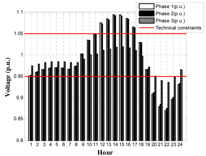
Fig. 5. Highest voltage values in each phase for baseline scenario.
