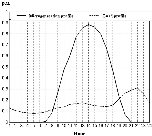
Fig. 4. Microgeneration and load profiles.
