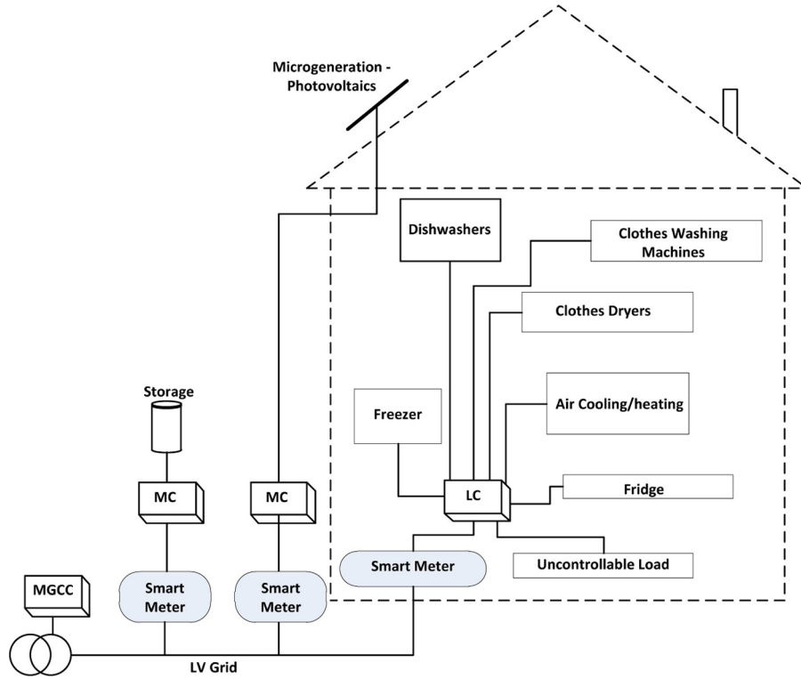
Fig. 1. Proposed control LV architecture for residential customers.
