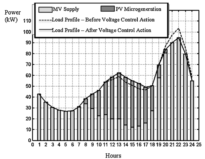
Fig. 9. Balance of power before/after voltage control action.
