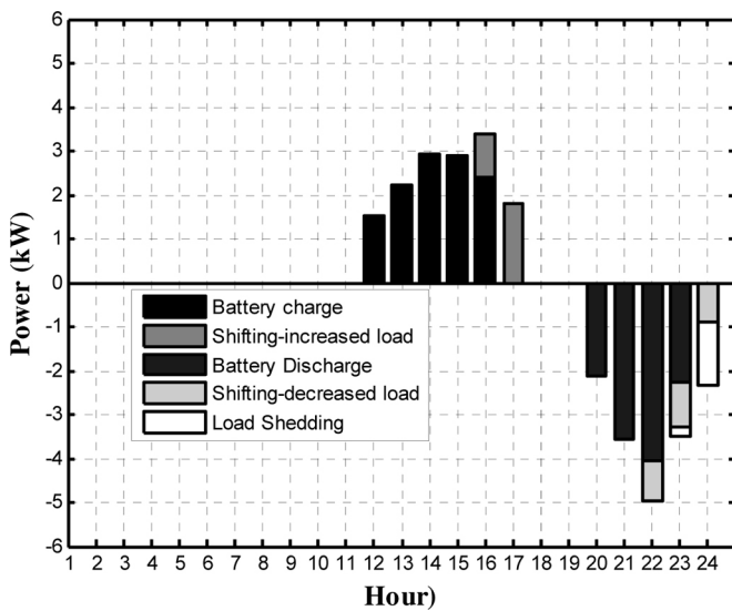
Fig. 7. Control actions performed in phase 1.
