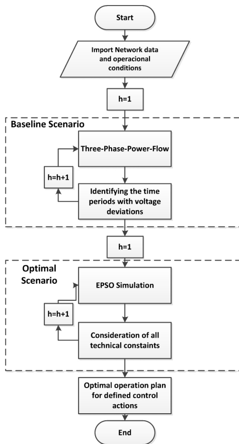
Fig. 2. Voltage control algorithm.
